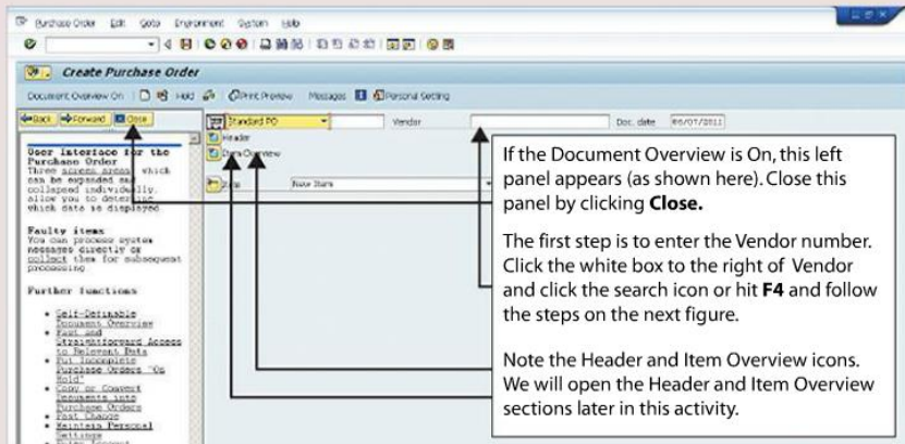
FIGURE 7A-4 Create Purchase Order Screen
